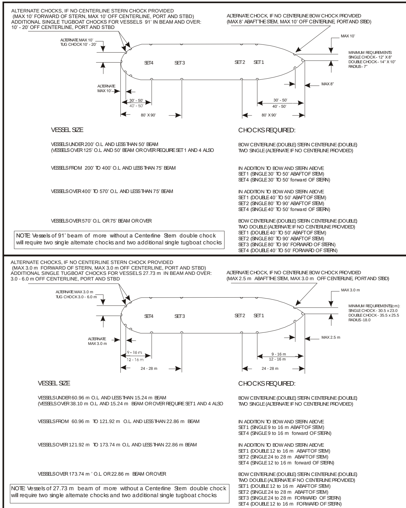
FIGURE 6 – Location of Chocks and Bitts (Panamax)
